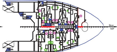
- 2-FORCASTLE DECK
