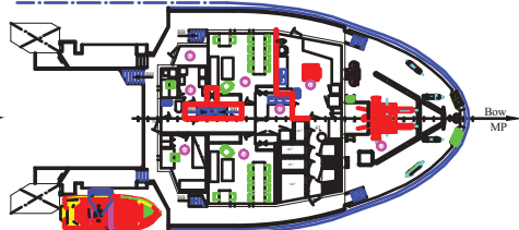
- MAIN DECK
